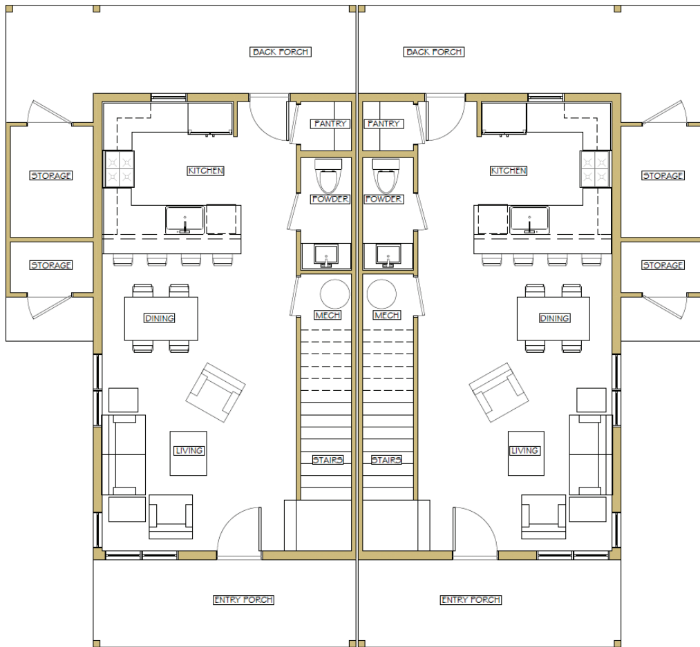
First Floor
