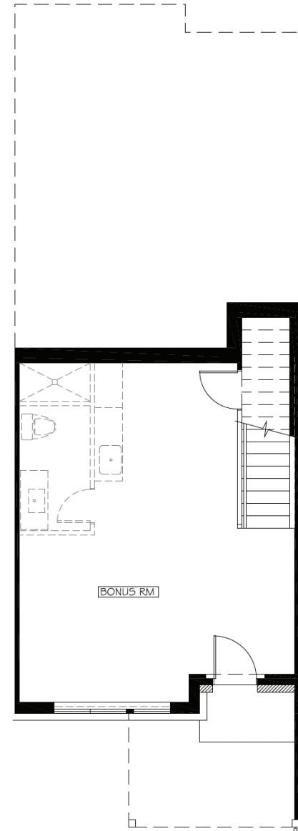
Lower Floor
